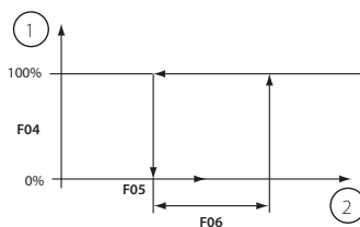
Cooling ON/OFF
