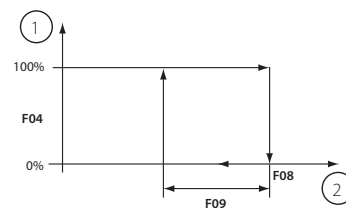
Heating ON/OFF
